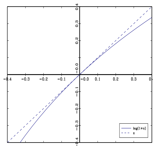
Figure 2.4: \log(1+x)
